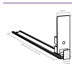
FORTA MAGNA-1 Pusher with big straight back support and small front
