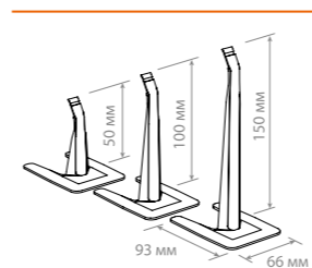
PC-STAND Price cassette stand
