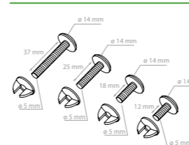
VIKING SCREW Plastic screw
