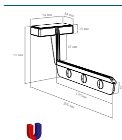
MGT-SGT-GP Magnetic sign holder with rivets
