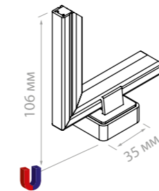
ALU-BOARD-MGT Aluminum sign holder with magnets
