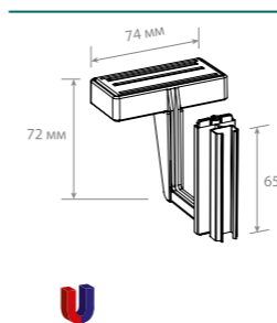
MAG-FLEX-PF Magnetic frame holder
