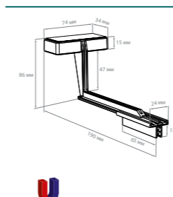
MGT-SGT-G Magnetic sign holder
