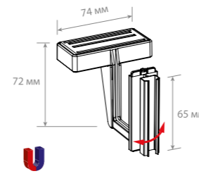
MAG-FLEX-PF Vertical plastic frame holder with strong magnet
