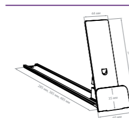
FORTA GROSSA-3 Pusher with big inclined back support and medium inclined front
