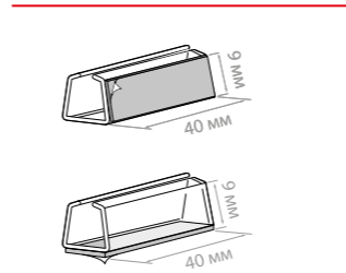
FLU-CLIP Clip with adhesive tape
