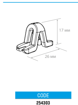
GRIPPER-CLIP Suspension loop for GRIPPER profile
