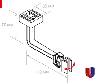
MGT-SW Swivel magnetic holder
