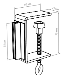
CLAMP SGT Metal clamp with supergrip holder
