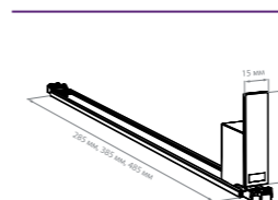
FORTA SLIMA-0 Slim pusher with high back support
