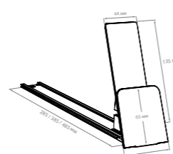
FORTA GROSSA-4 Pusher with high inclined back support and big inclined front
